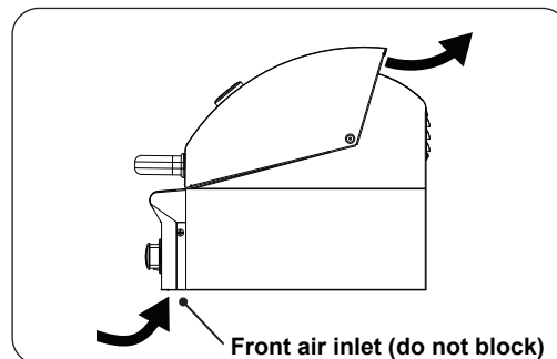
Fig. 16-1 Airflow diagram
