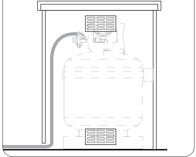
Fig. 25-1 L.P. Cylinder enclosure construction overview (if applicable)
