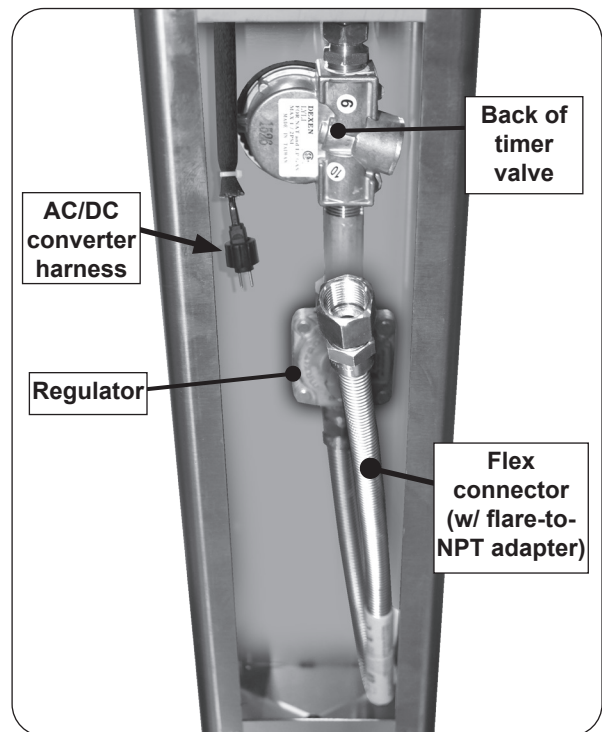
Fig. 26-2 Post interior detail
