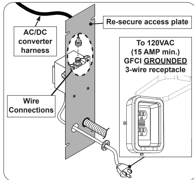
Fig. 28-1 Connect: Wires, Plate, Power
