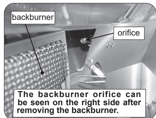
Fig. 46-4 Remove backburner
