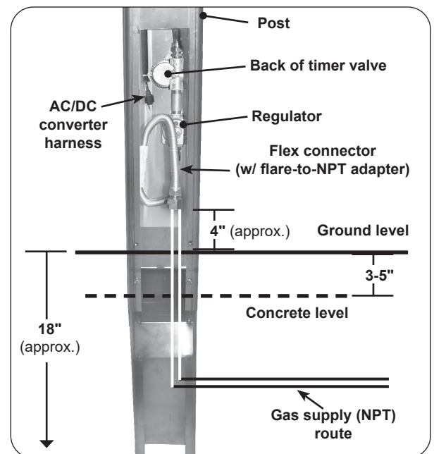
Fig. 29-2 In-ground install orientation
