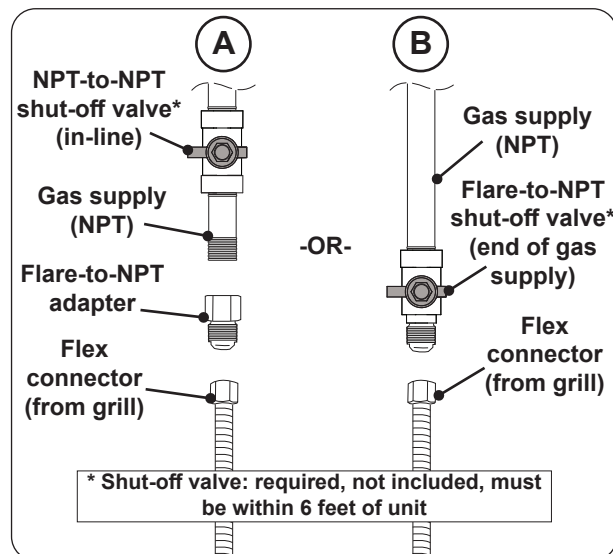
Fig. 31-1 Connecting to a gas line
