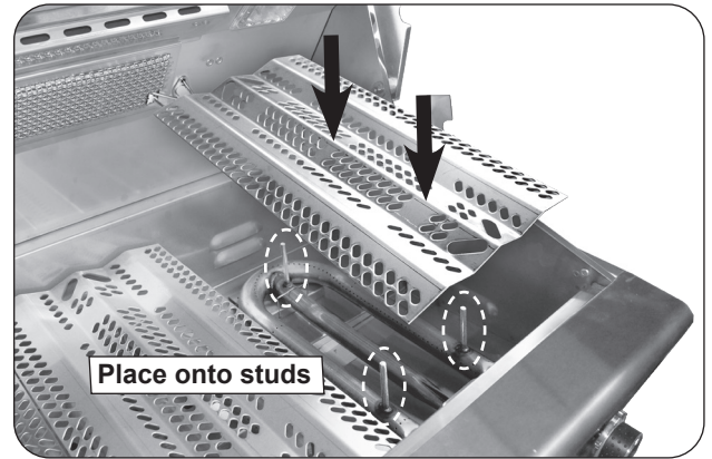
Fig. 33-1 Install vaporizer panels
