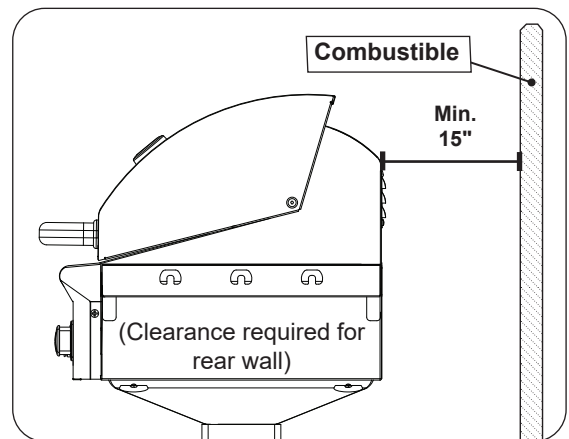
Fig. 14-3 Clearance 'C' Diagram
