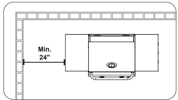
Fig. 15-1 Corner wall clearance
