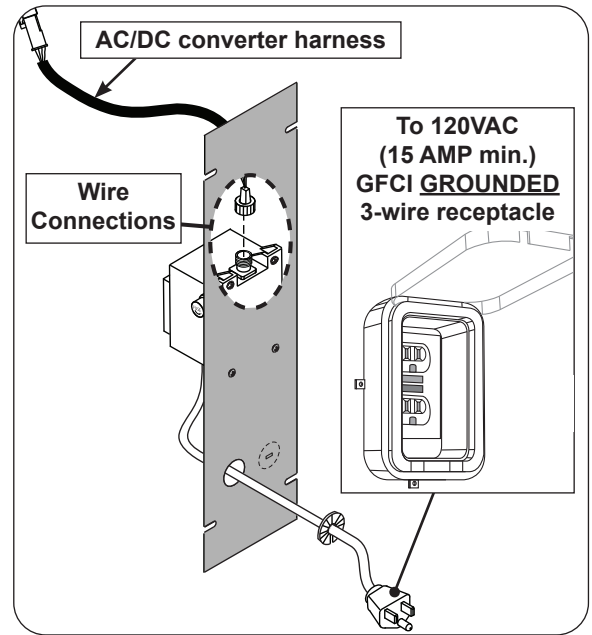
Fig. 32-1 Connect: Wires, Plate, Power
