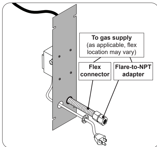
Fig. 27-1 Flex connector detail
