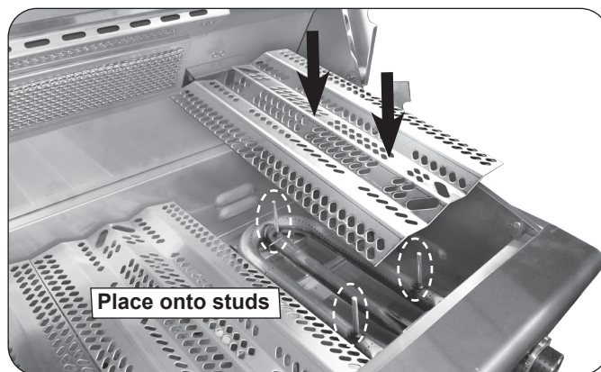
Fig. 28-1 Install vaporizer panels
