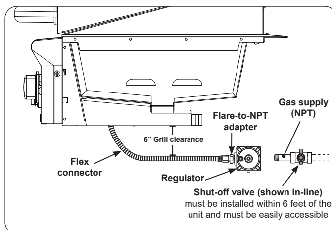
Fig. 27-2 Connecting to a gas line
