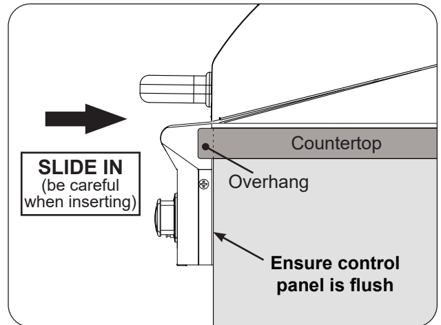
Fig. 26-2 Slide in unit (ensure flush)
