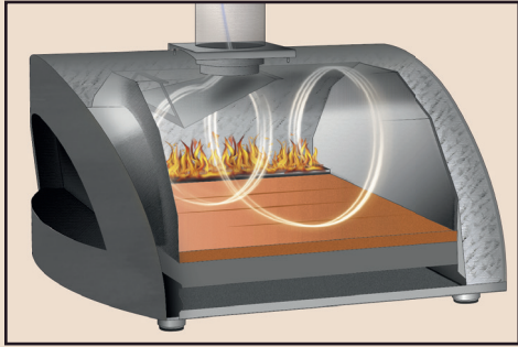
03 Patented Full Effect Full Circulation Flue System™
