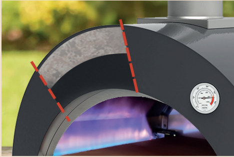
02 DoubleDown Ceramic Superwool® Insulation
