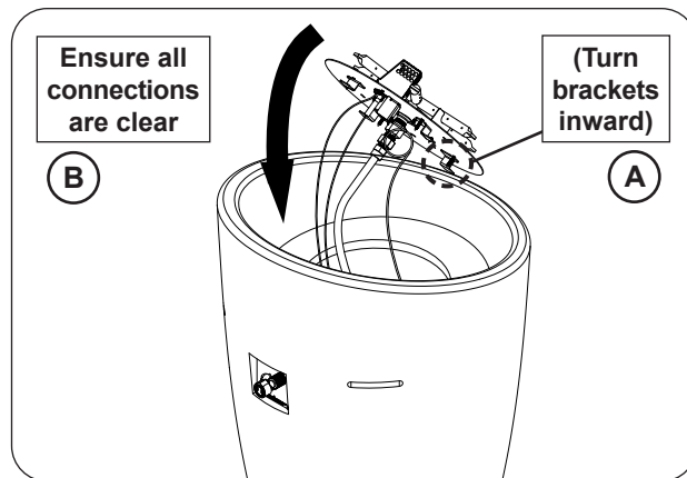
Fig. 22-1 Insert burner assembly
