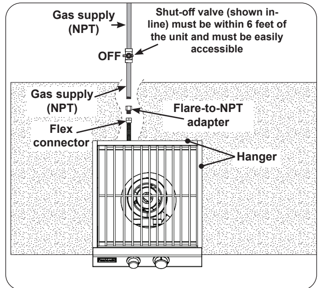
Fig. 28-2 Household propane & nat. gas diagram
