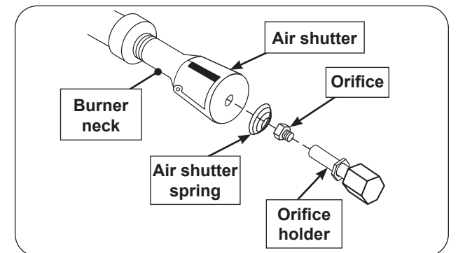
Fig. 40-3 Burner replacement diagram
