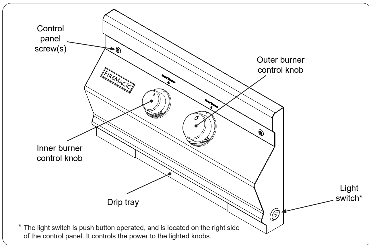
Fig. 33-1 Power burner controls
