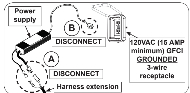
Fig. 40-4 Perform system reset
