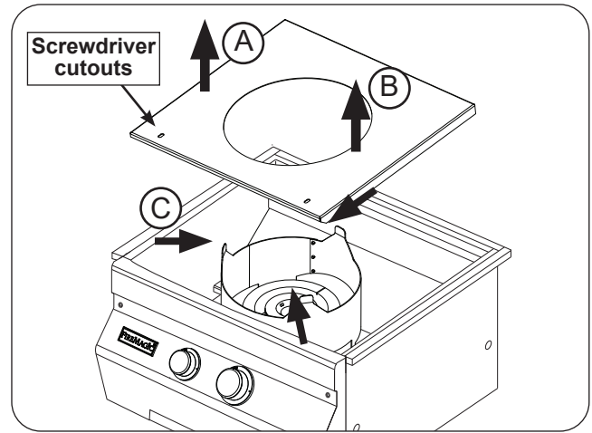
Fig. 40-1 Interior protection plate removal
