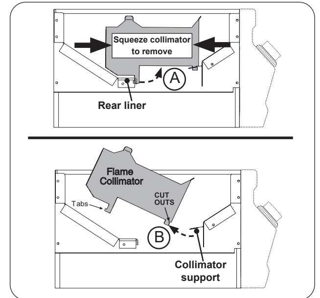
Fig. 40-2 Flame collimator removal
