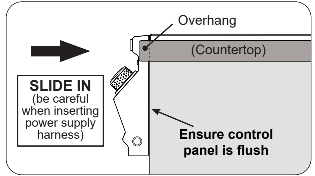
Fig. 27-1 Slide in unit (ensure flush)
