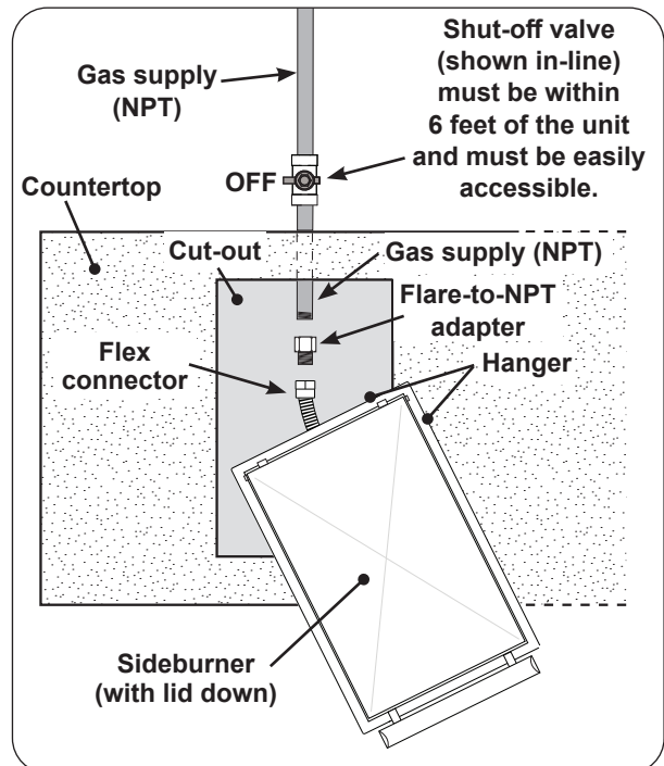
Fig. 24-3 Household propane and natural gas diagram
