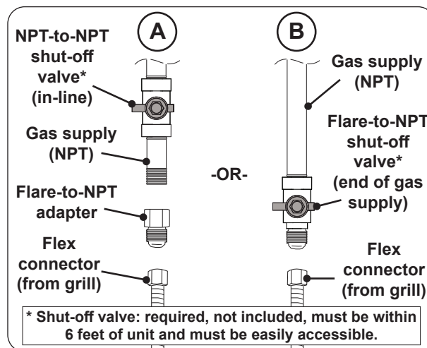
Fig. 26-2 Connecting to a gas line
