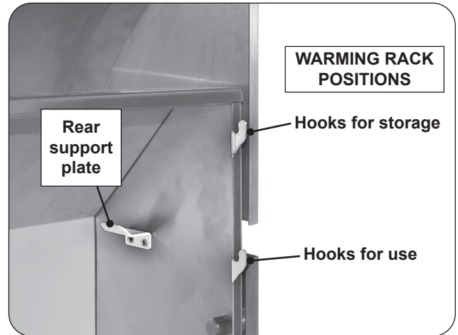
Fig. 28-1 Warming rack hooks
