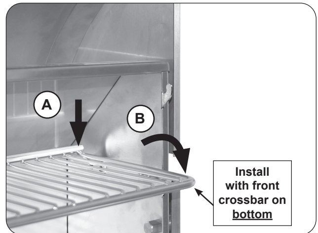
Fig. 28-2 Place warming rack for use
