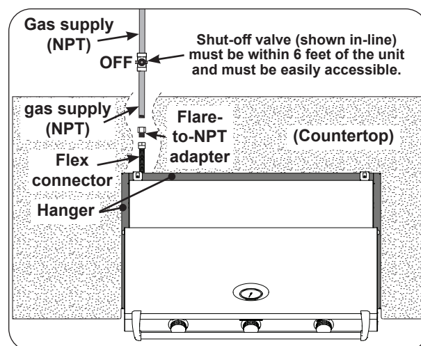
Fig. 26-3 Household LP & Nat. gas diagram
