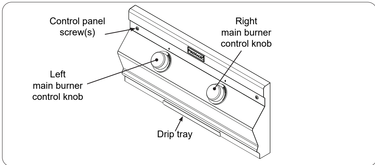
Fig. 30-1 CM430i controls
